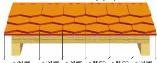
Installation using independent verge tiles
