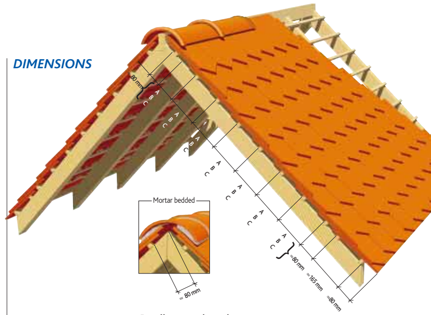
Installation with overhanging verges
