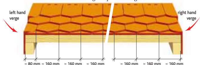
Installation using independent verge tiles
