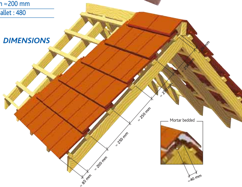
Installation without independent verge tiles
