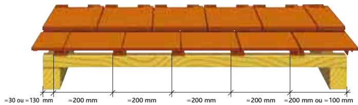
Installation using independent verge tiles
