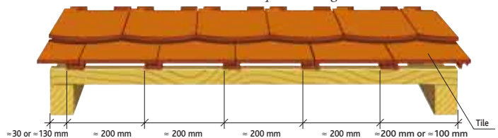
Installation without independent verge tiles
