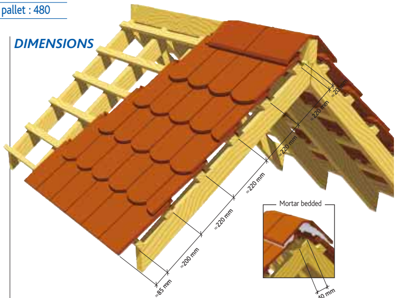
Installation without independent verge tiles
