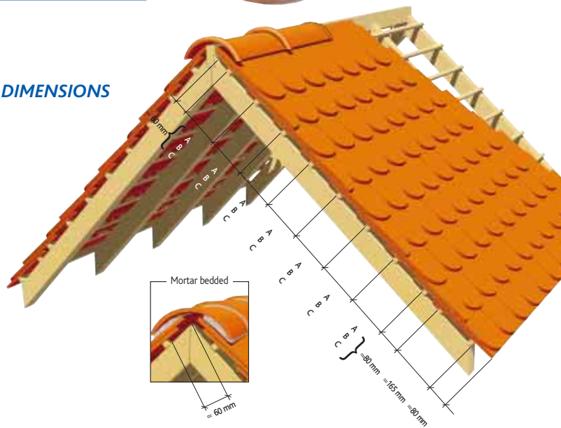
Installation with overhanging verge
