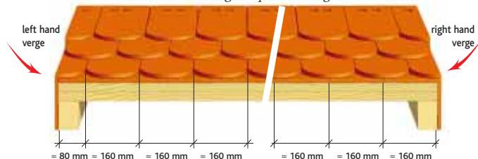
Installation using independent verge tiles
