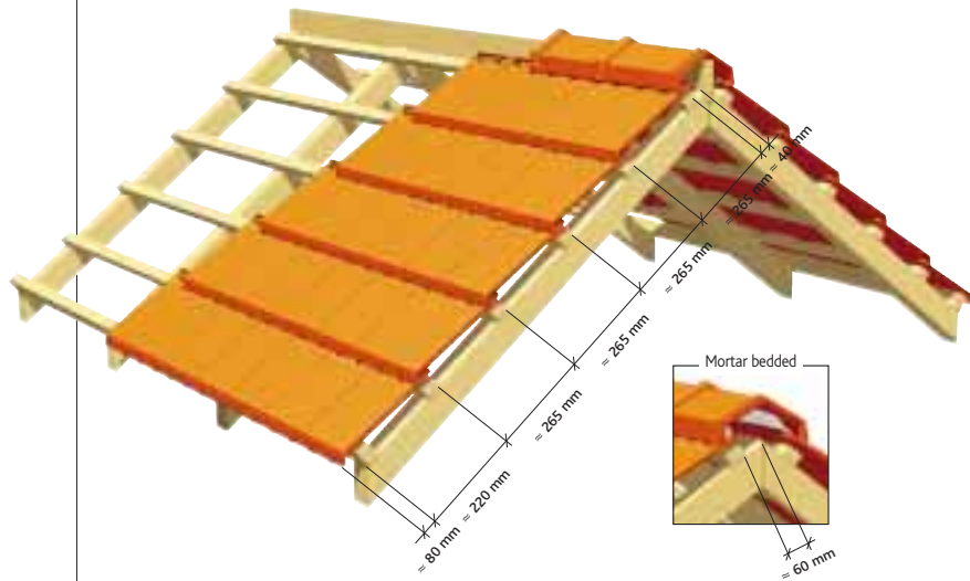
Installation using independent verge tiles
