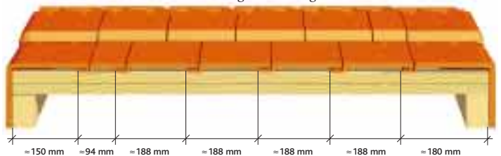
Installation using cloaked verge tiles
