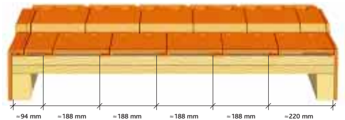
Installation using cloaked verge tiles
